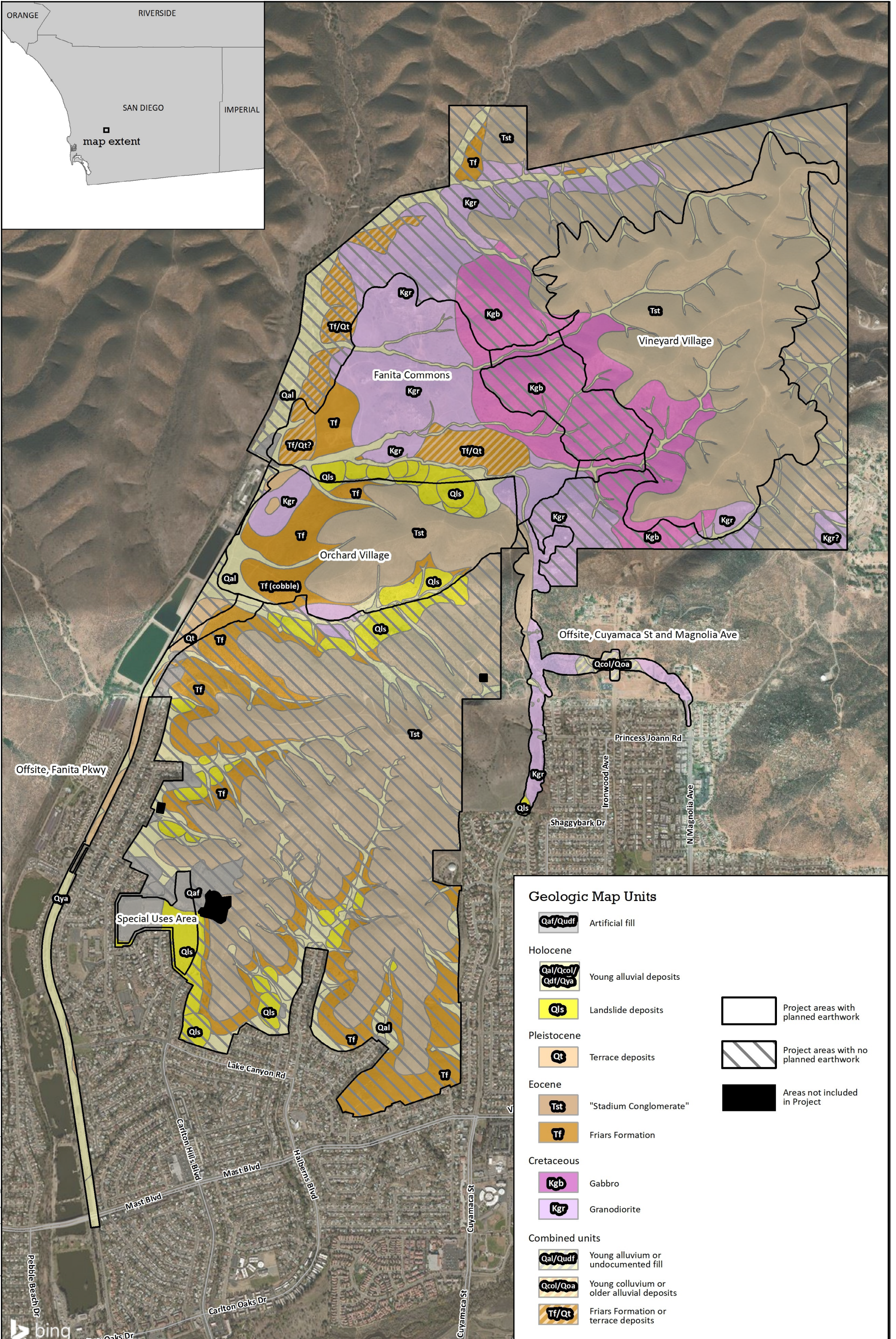
Figure 4.6-1 Geologic Map of the Project Site
